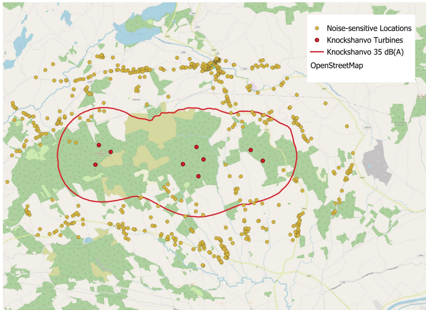
Figure 1 Noise Contour at 35 dB due to Knockshanvo Wind Farm
